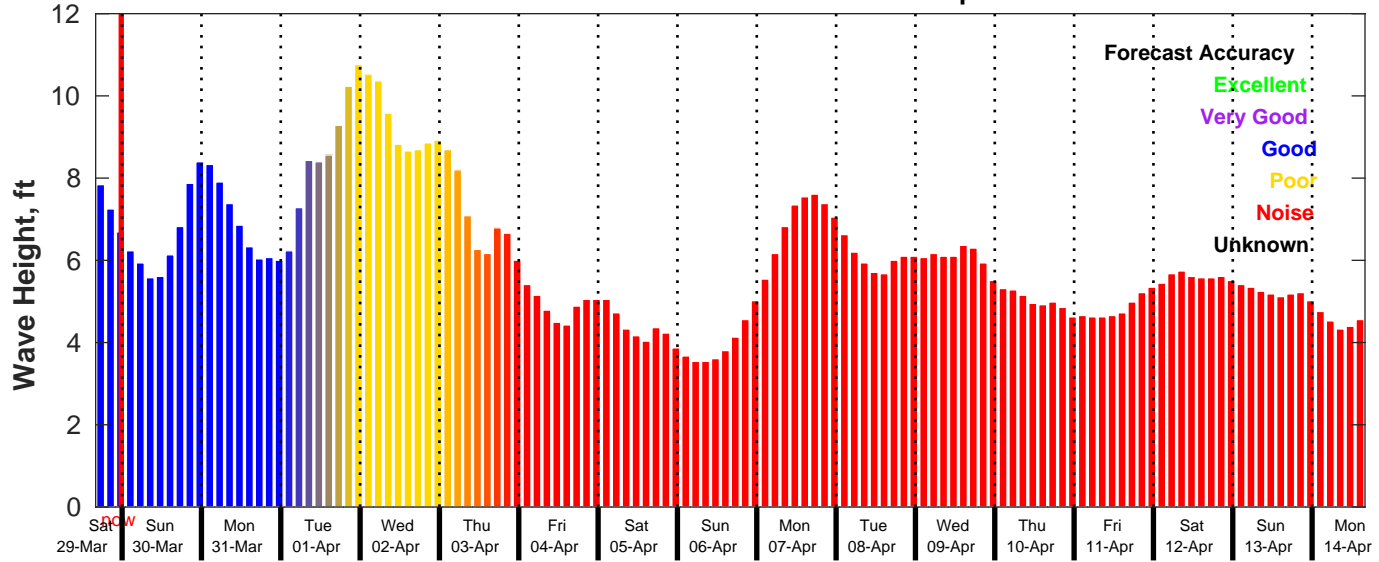
GFS Wave Forecast for NDBC 46011 from 29-Mar-2025 16:00:00 to 14-Apr-2025 16:00:00
