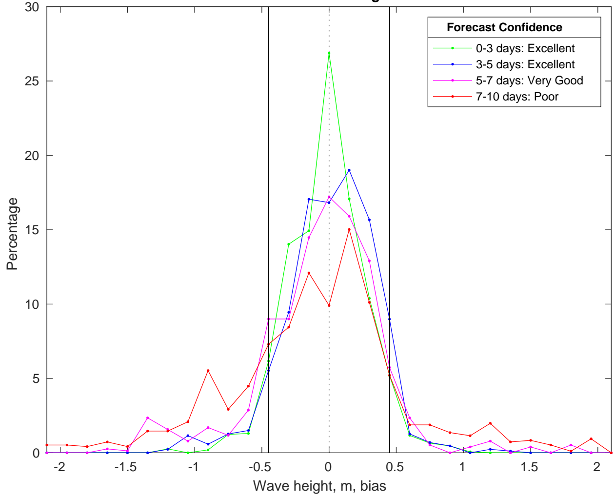
NDBC 46028 vs CMEMS Waves Bias Histogram: 30-Mar-2025
