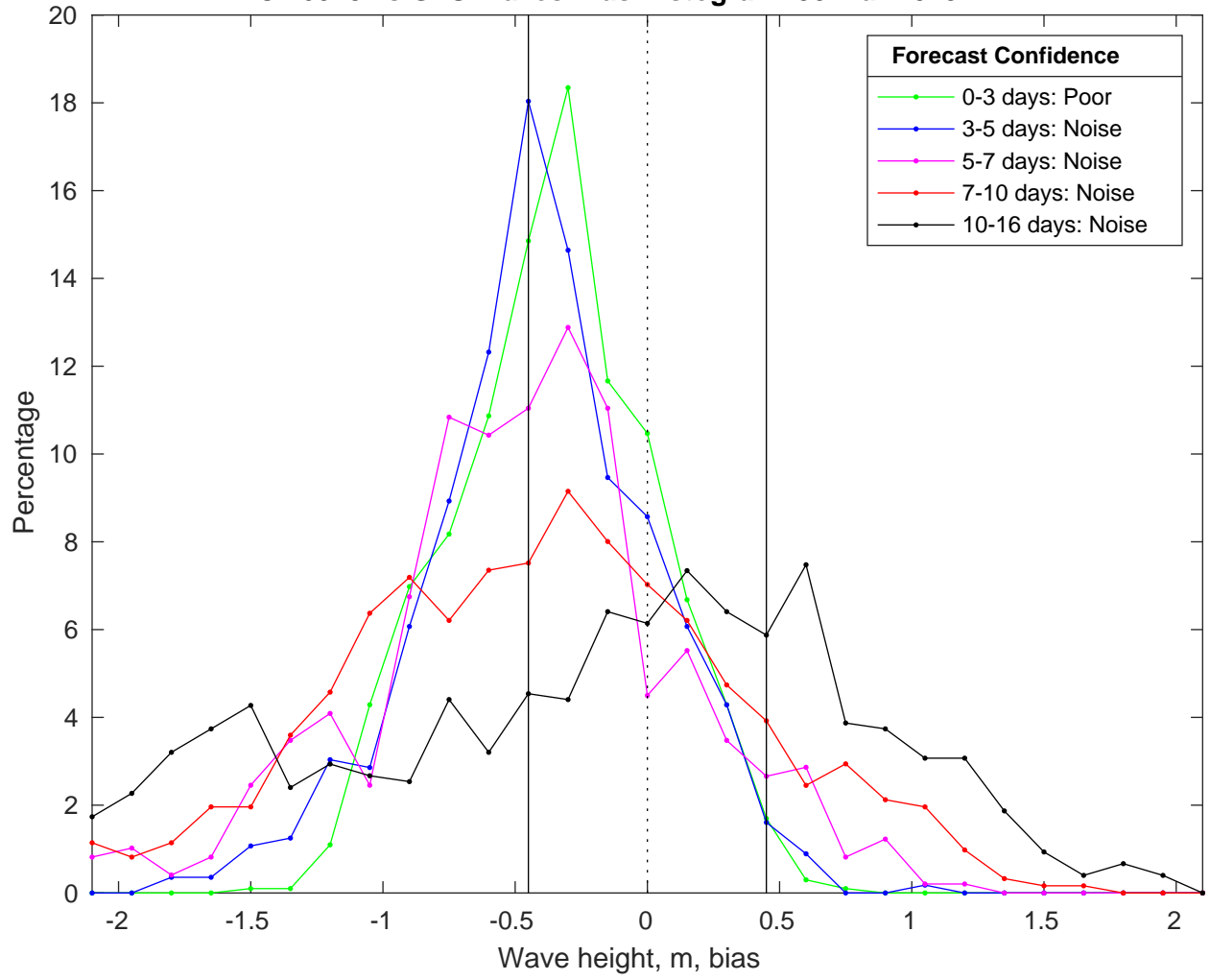
NDBC 46028 vs GFS Waves Bias Histogram: 30-Mar-2025
