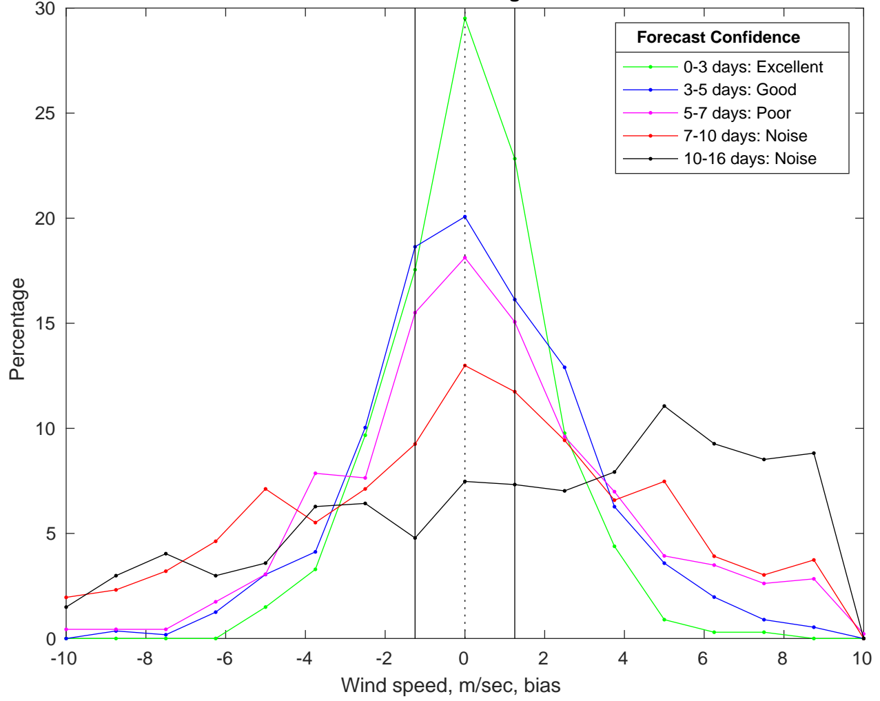
NDBC 46028 vs GFS Winds Bias Histogram: 30-Mar-2025
