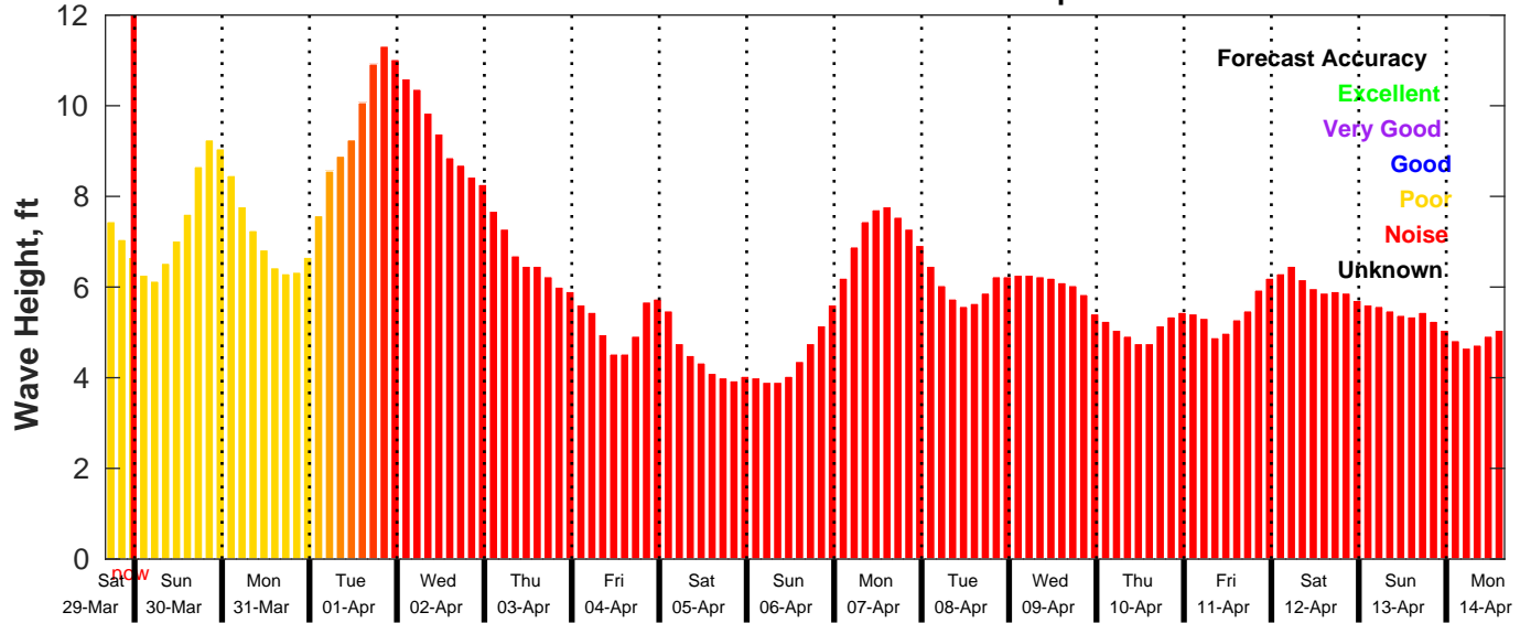
GFS Wave Forecast for NDBC 46028 from 29-Mar-2025 16:00:00 to 14-Apr-2025 16:00:00
