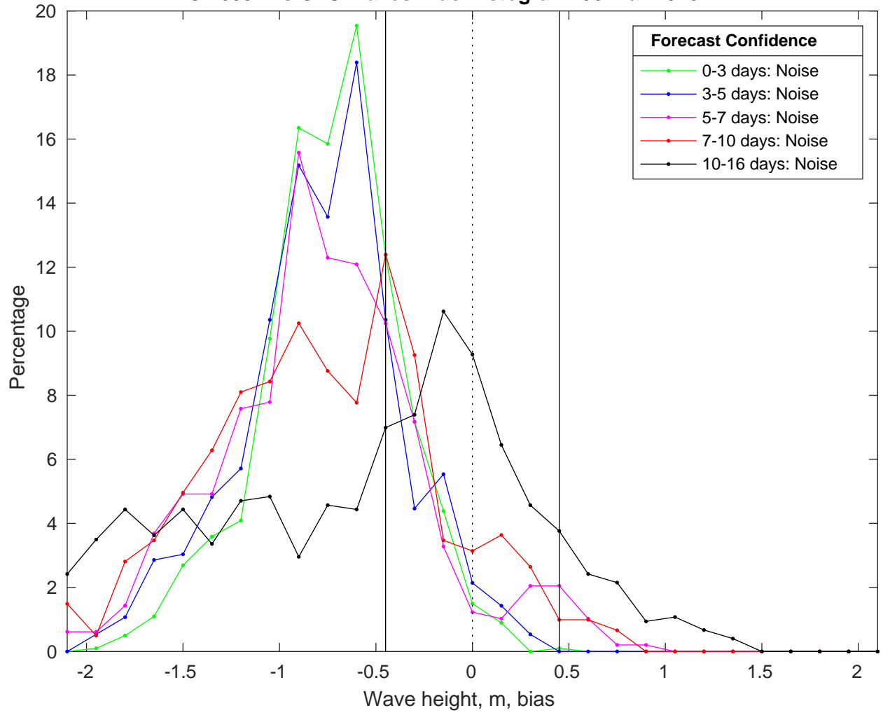
NDBC 46054 vs GFS Waves Bias Histogram: 30-Mar-2025
