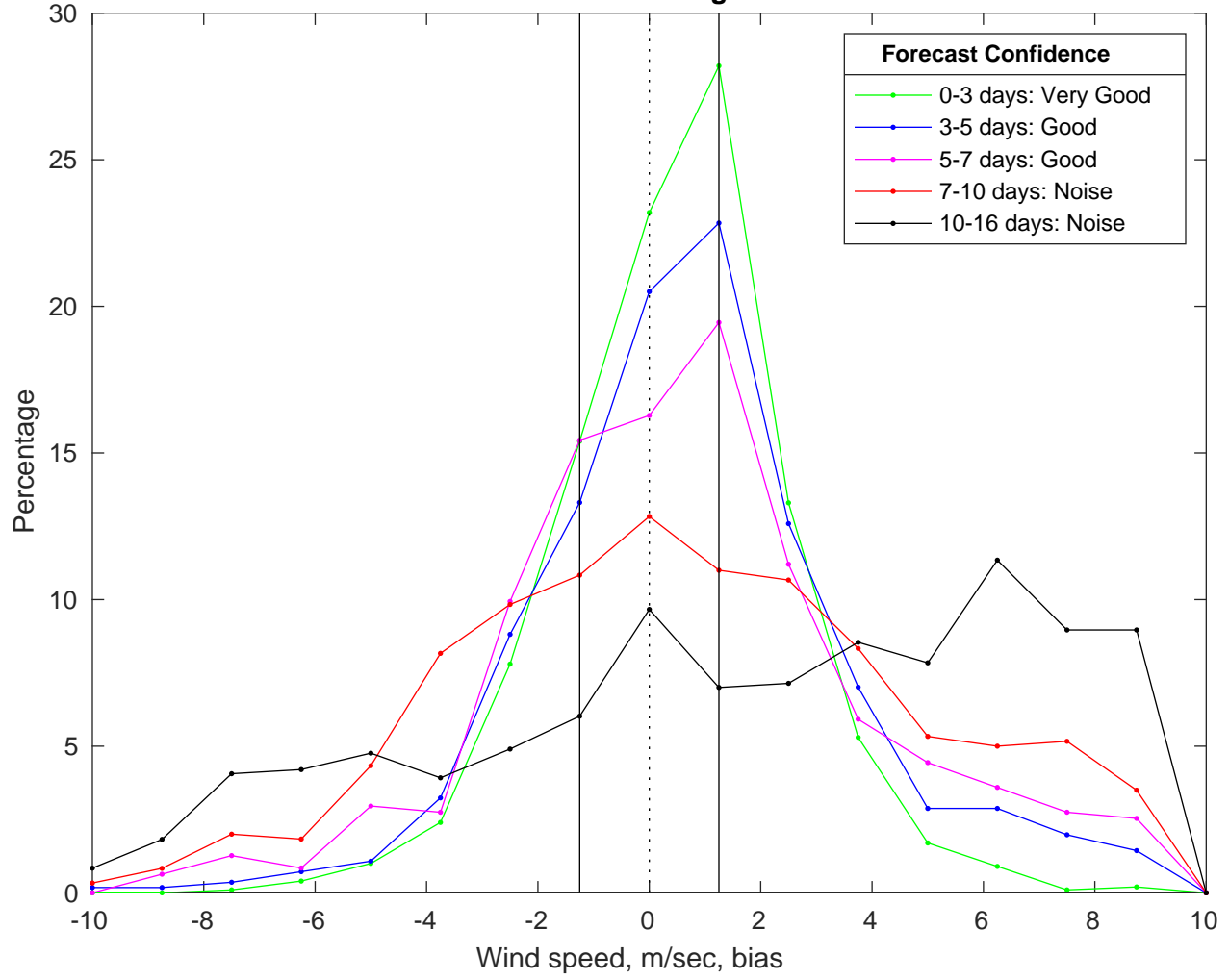
NDBC 46054 vs GFS Winds Bias Histogram: 30-Mar-2025
