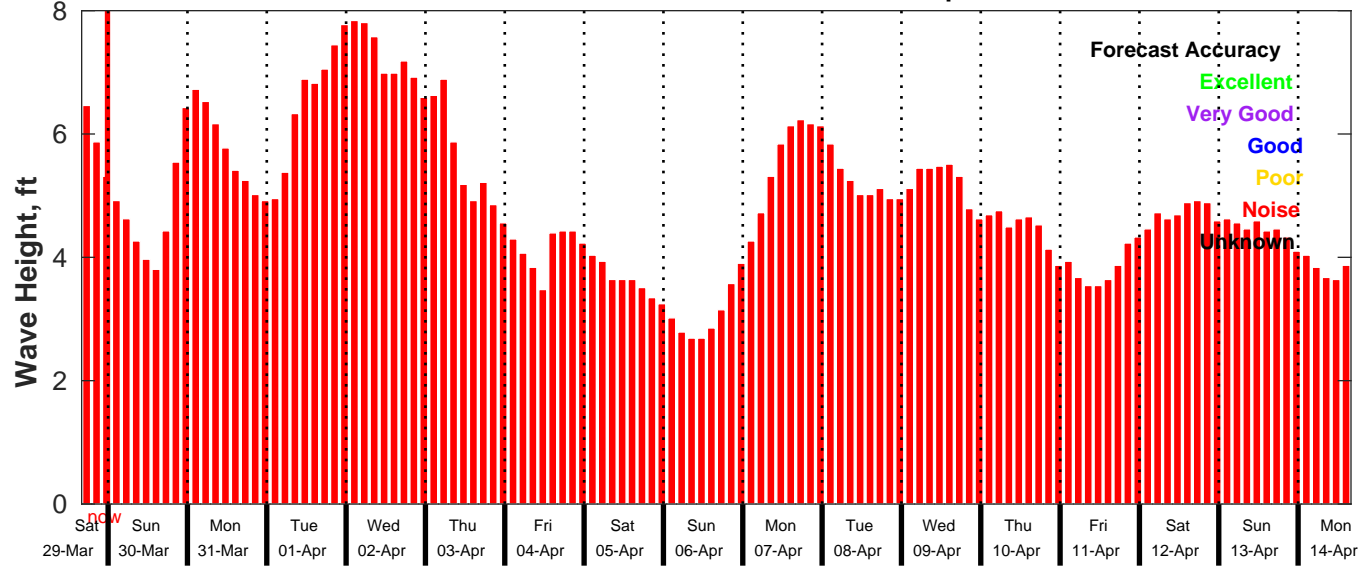
GFS Wave Forecast for NDBC 46054 from 29-Mar-2025 16:00:00 to 14-Apr-2025 16:00:00
