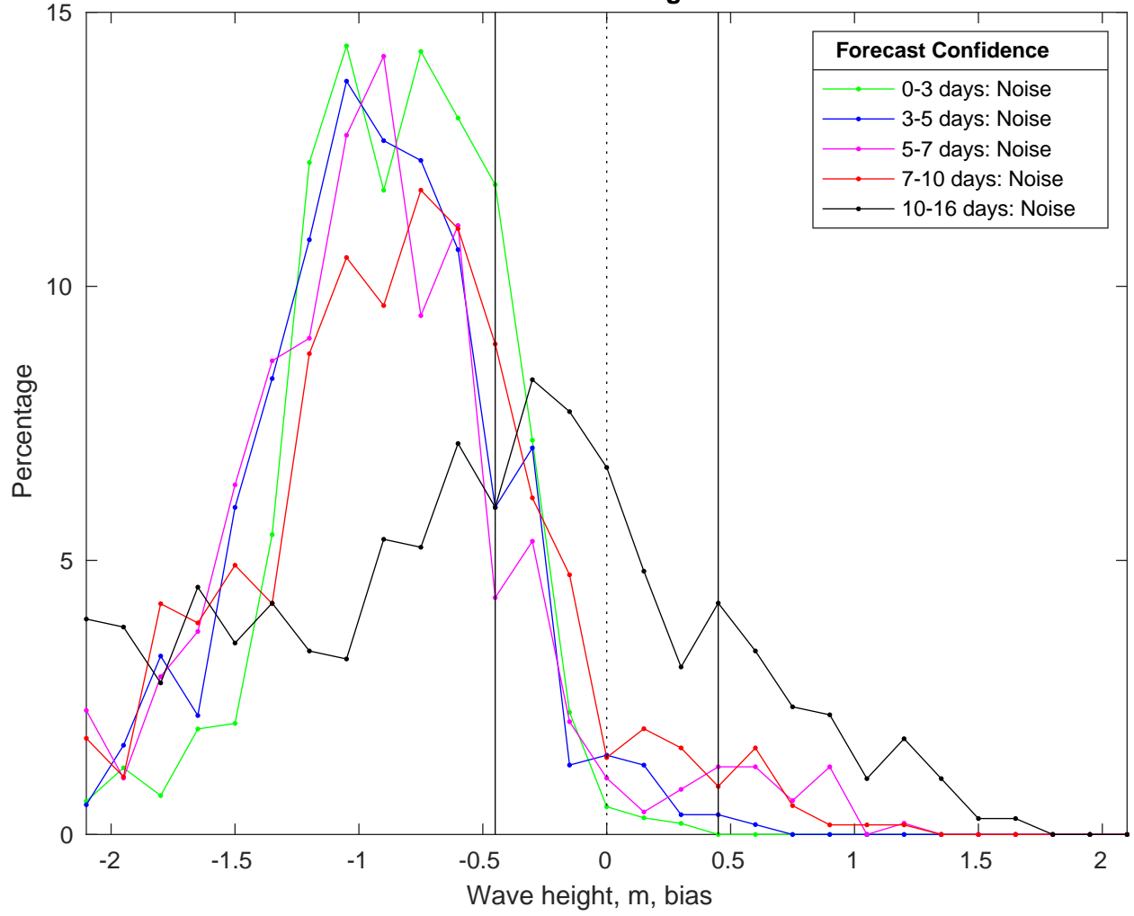
NDBC 46069 vs GFS Waves Bias Histogram: 30-Mar-2025
