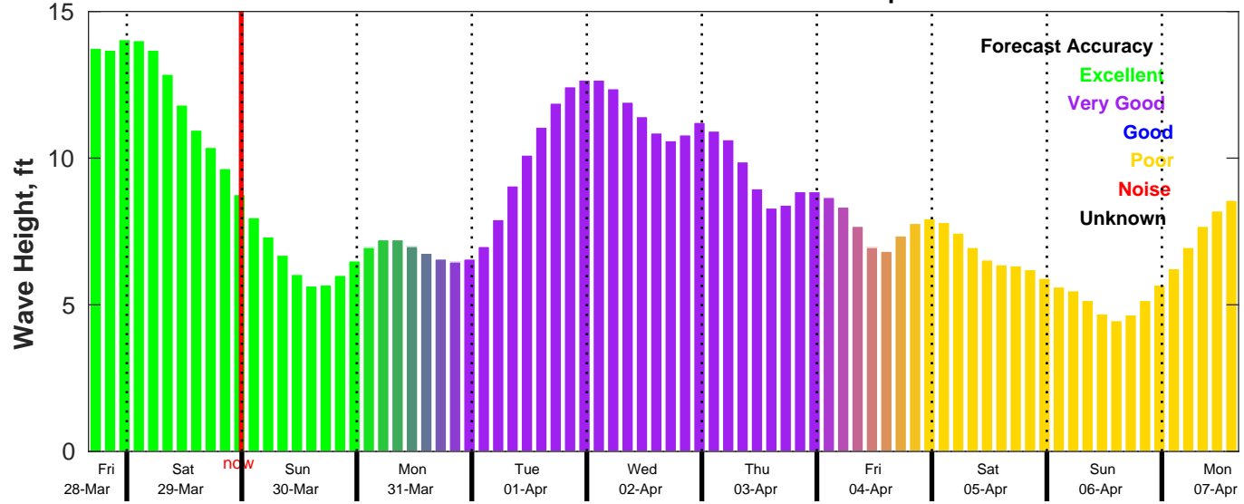
CMEMS Wave Forecast for NDBC 46069 from 28-Mar-2025 16:00:00 to 07-Apr-2025 16:00:00
