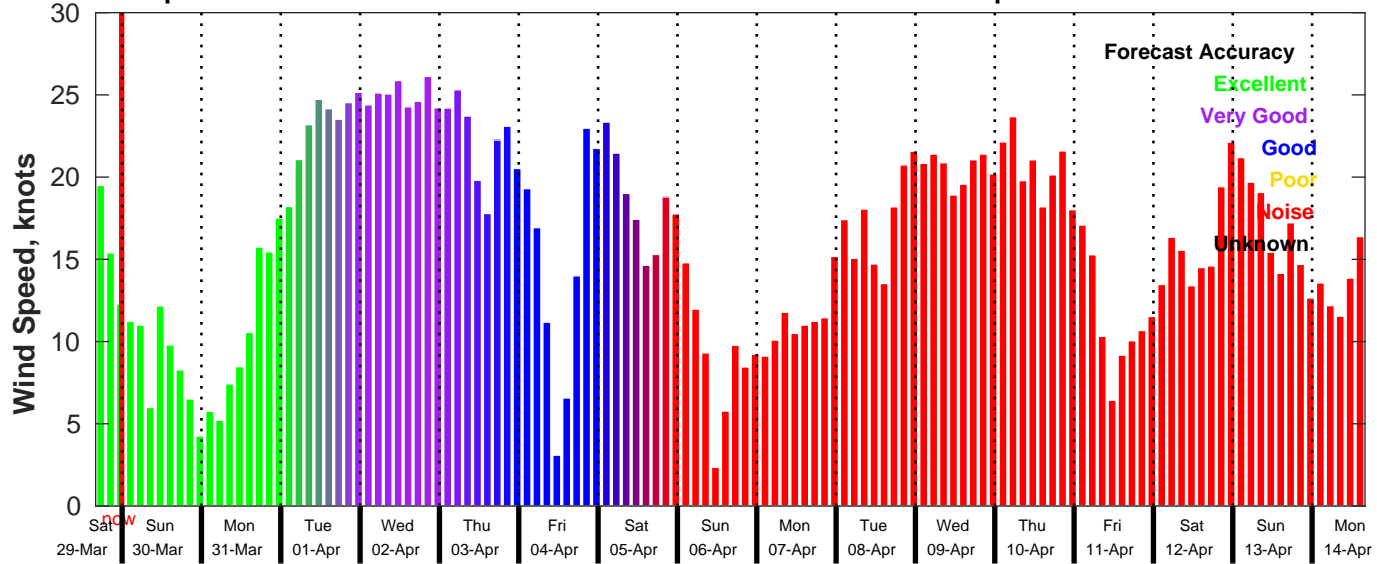
GFS Wind Speed Forecast for NDBC 46069 from 29-Mar-2025 16:00:00 to 14-Apr-2025 16:00:00
