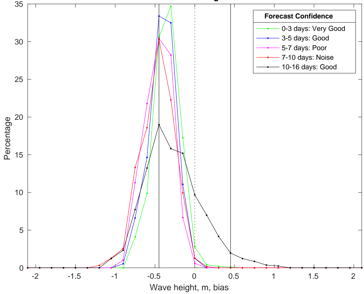
NDBC 51209 vs GFS Waves Bias Histogram: 30-Mar-2025
