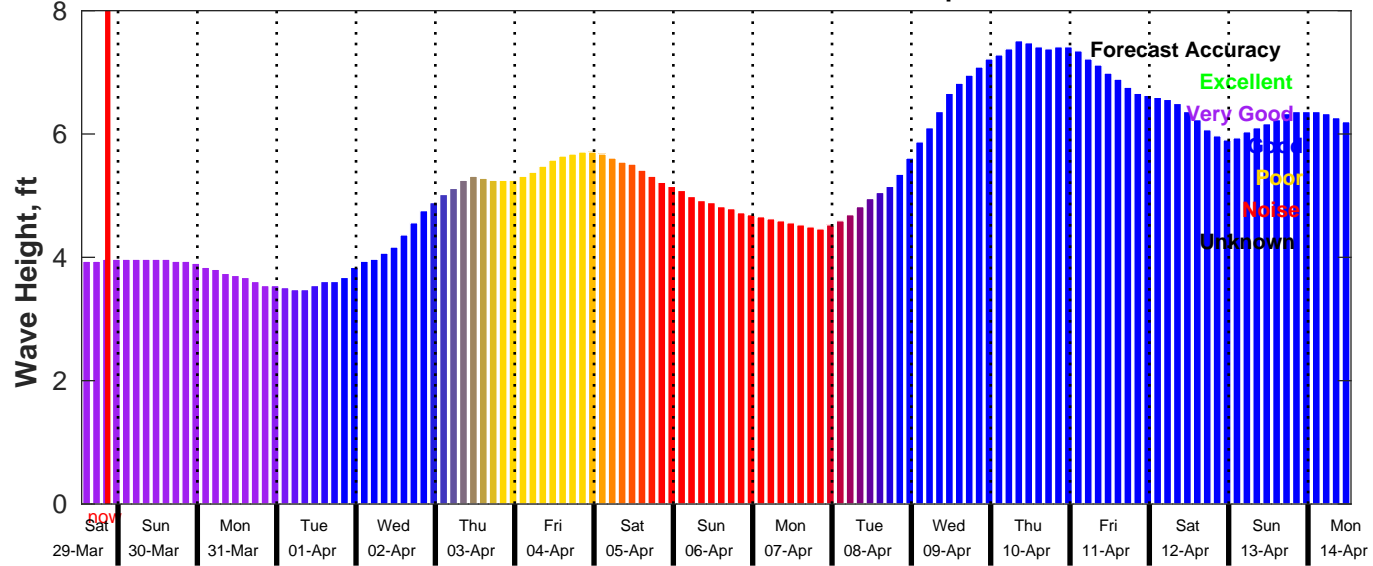
GFS Wave Forecast for NDBC 51209 from 29-Mar-2025 13:00:00 to 14-Apr-2025 13:00:00
