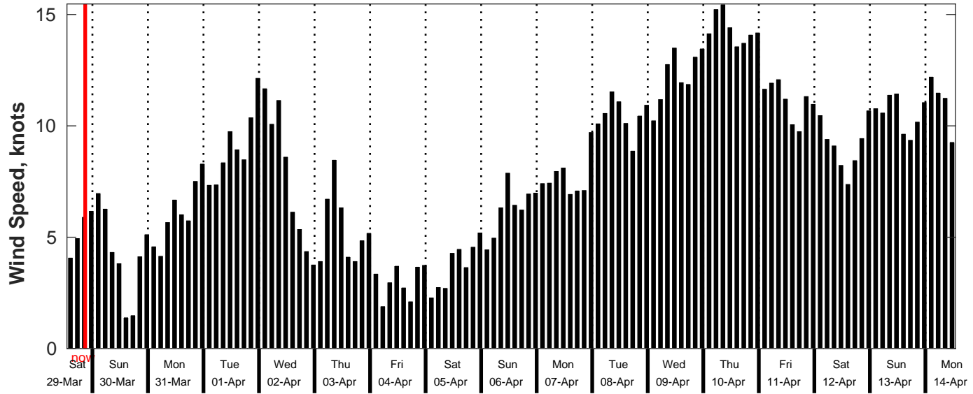
GFS Wind Speed Forecast for NDBC 51209 from 29-Mar-2025 13:00:00 to 14-Apr-2025 13:00:00
