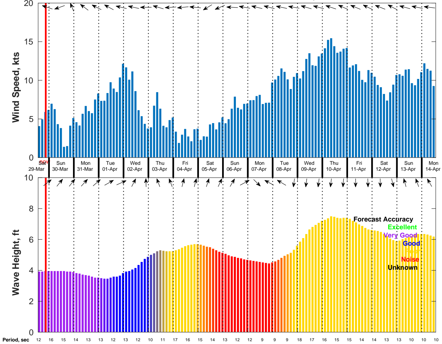
Wind & Wave Forecast for NDBC 51209 from 29-Mar-2025 13:00:00 to 14-Apr-2025 13:00:00
