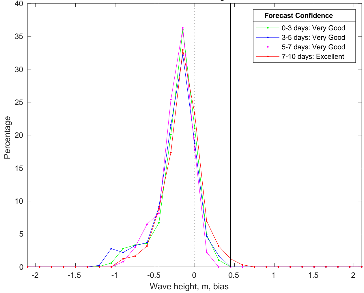
NDBC 52211 vs CMEMS Waves Bias Histogram: 30-Mar-2025
