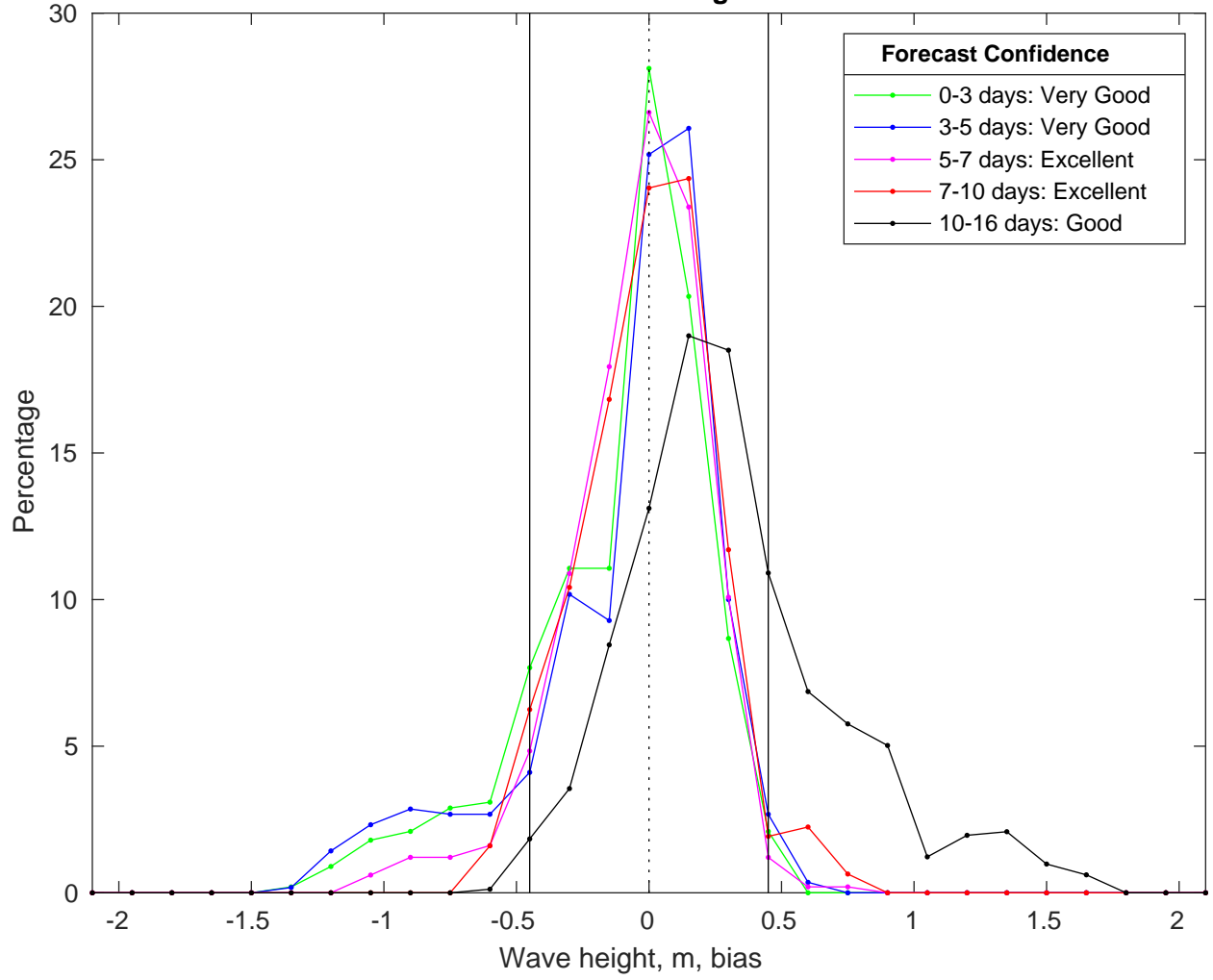
NDBC 52211 vs GFS Waves Bias Histogram: 30-Mar-2025
