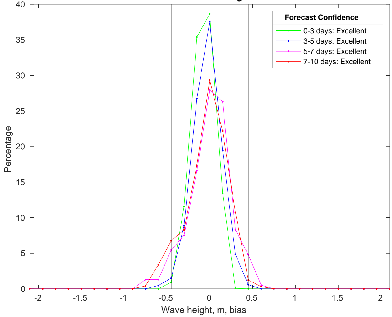
NDBC 52212 vs CMEMS Waves Bias Histogram: 30-Mar-2025
