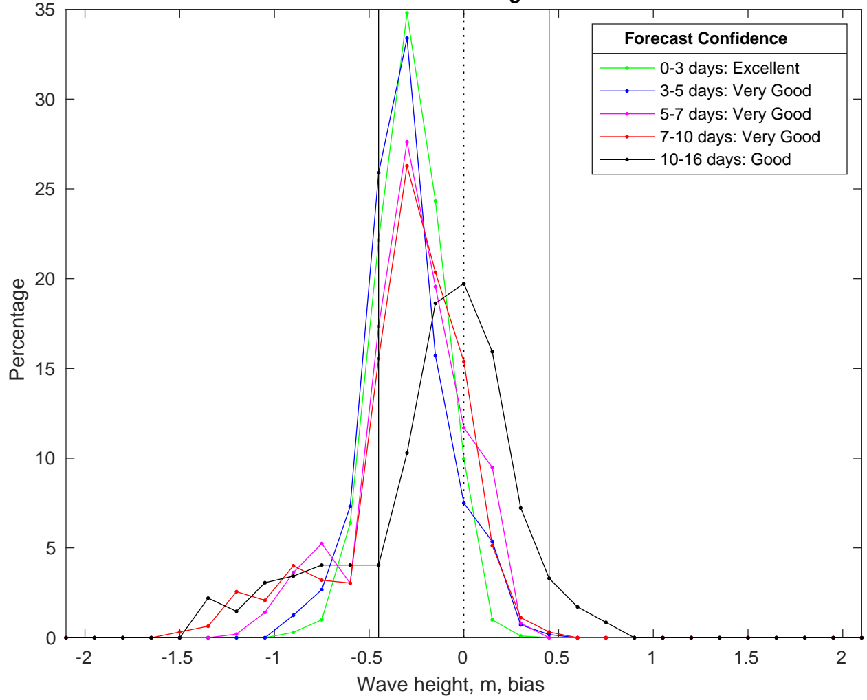
NDBC 52212 vs GFS Waves Bias Histogram: 30-Mar-2025
