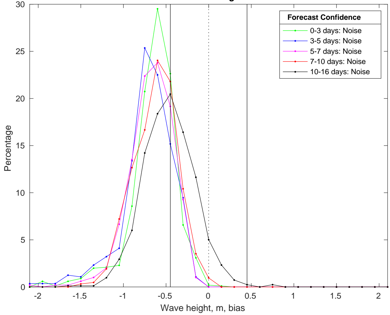
NDBC 52213 vs GFS Waves Bias Histogram: 30-Mar-2025
