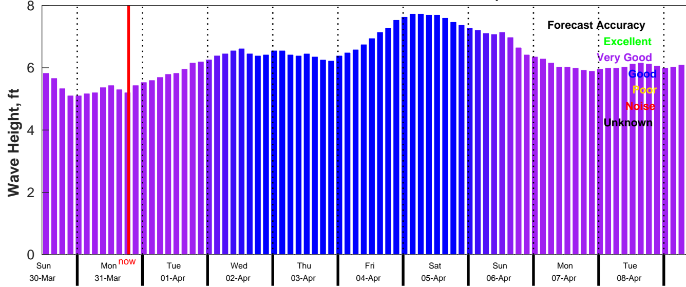
CMEMS Wave Forecast for NDBC 52213 from 29-Mar-2025 11:00:00 to 08-Apr-2025 11:00:00
