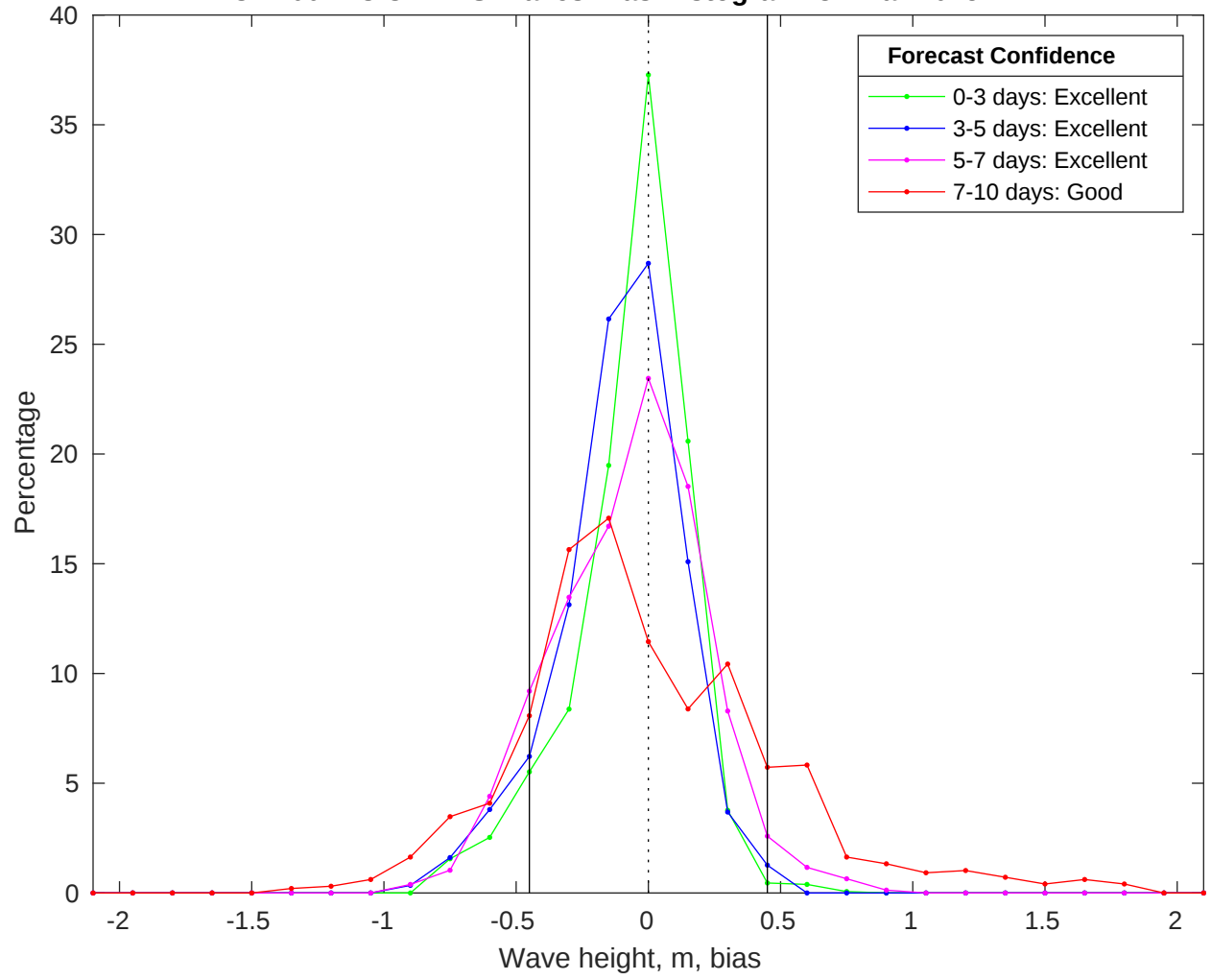
NDBC 41004 vs CMEMS Waves Bias Histogram: 31-Mar-2025
