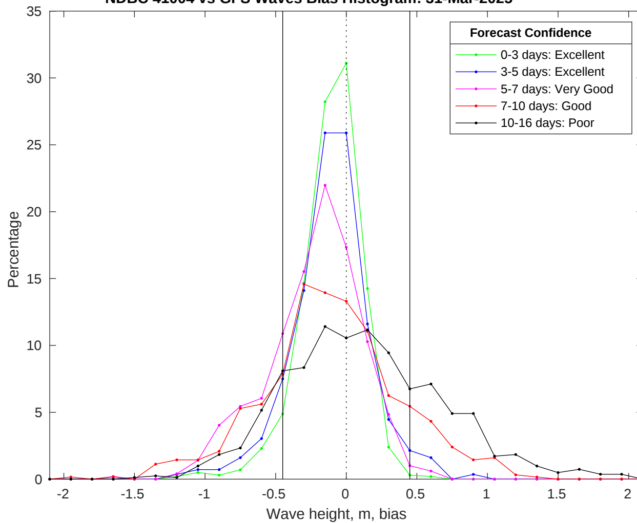
NDBC 41004 vs GFS Waves Bias Histogram: 31-Mar-2025
