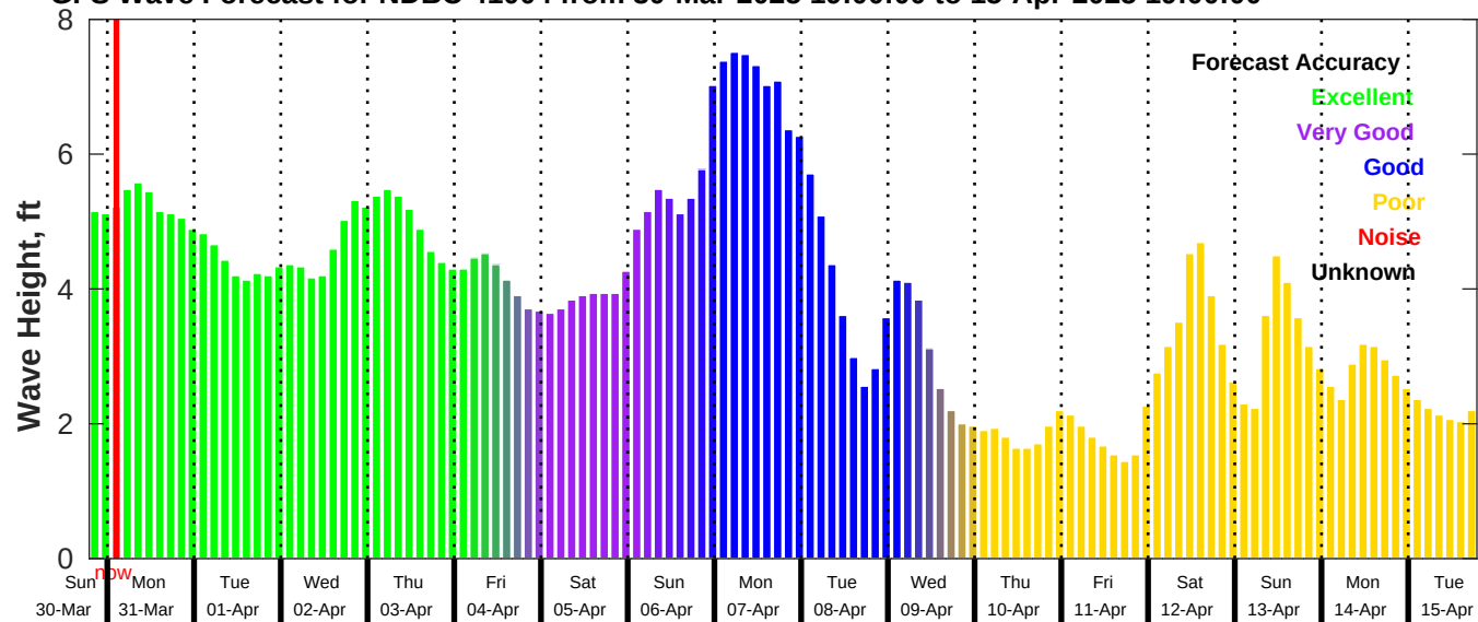
GFS Wave Forecast for NDBC 41004 from 30-Mar-2025 19:00:00 to 15-Apr-2025 19:00:00
