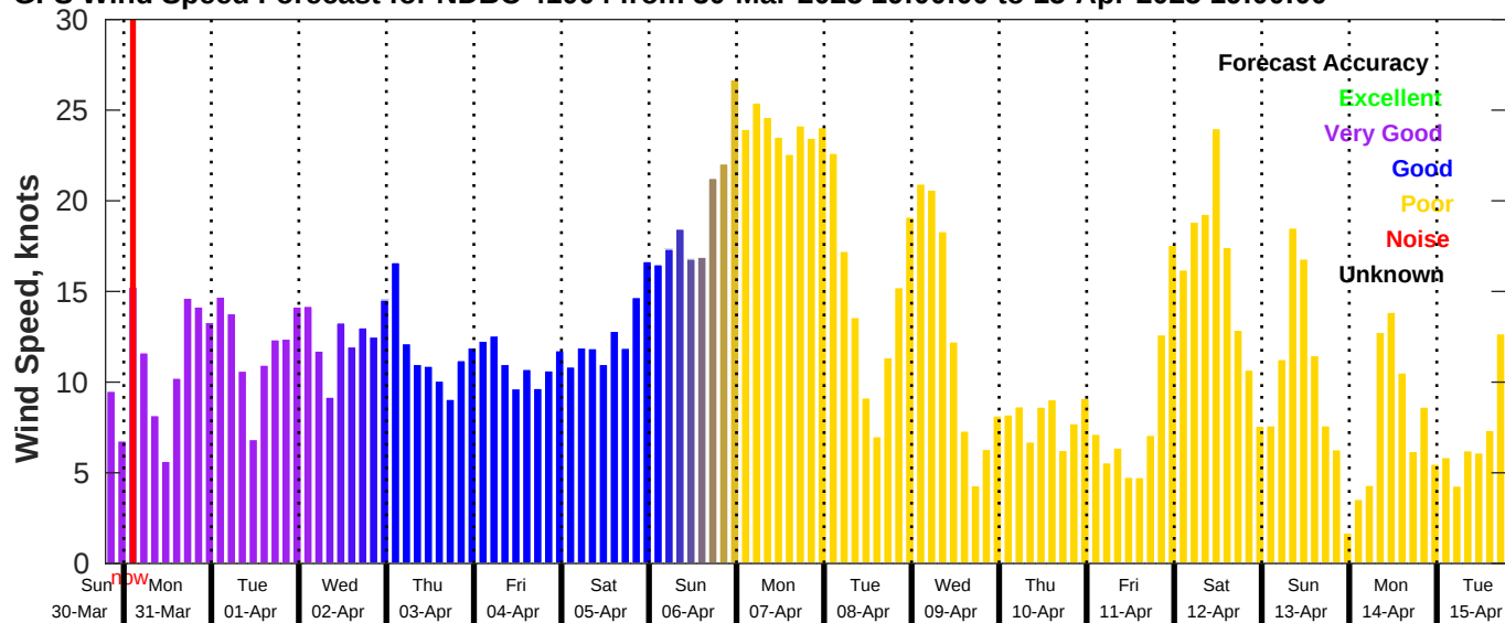
GFS Wind Speed Forecast for NDBC 41004 from 30-Mar-2025 19:00:00 to 15-Apr-2025 19:00:00
