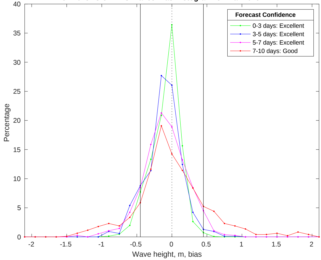
NDBC 41013 vs CMEMS Waves Bias Histogram: 31-Mar-2025
