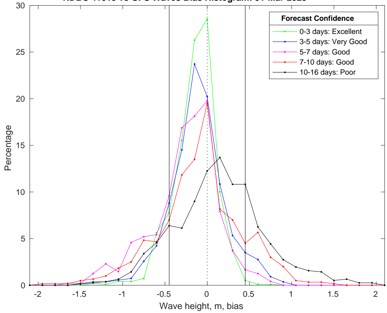
NDBC 41013 vs GFS Waves Bias Histogram: 31-Mar-2025
