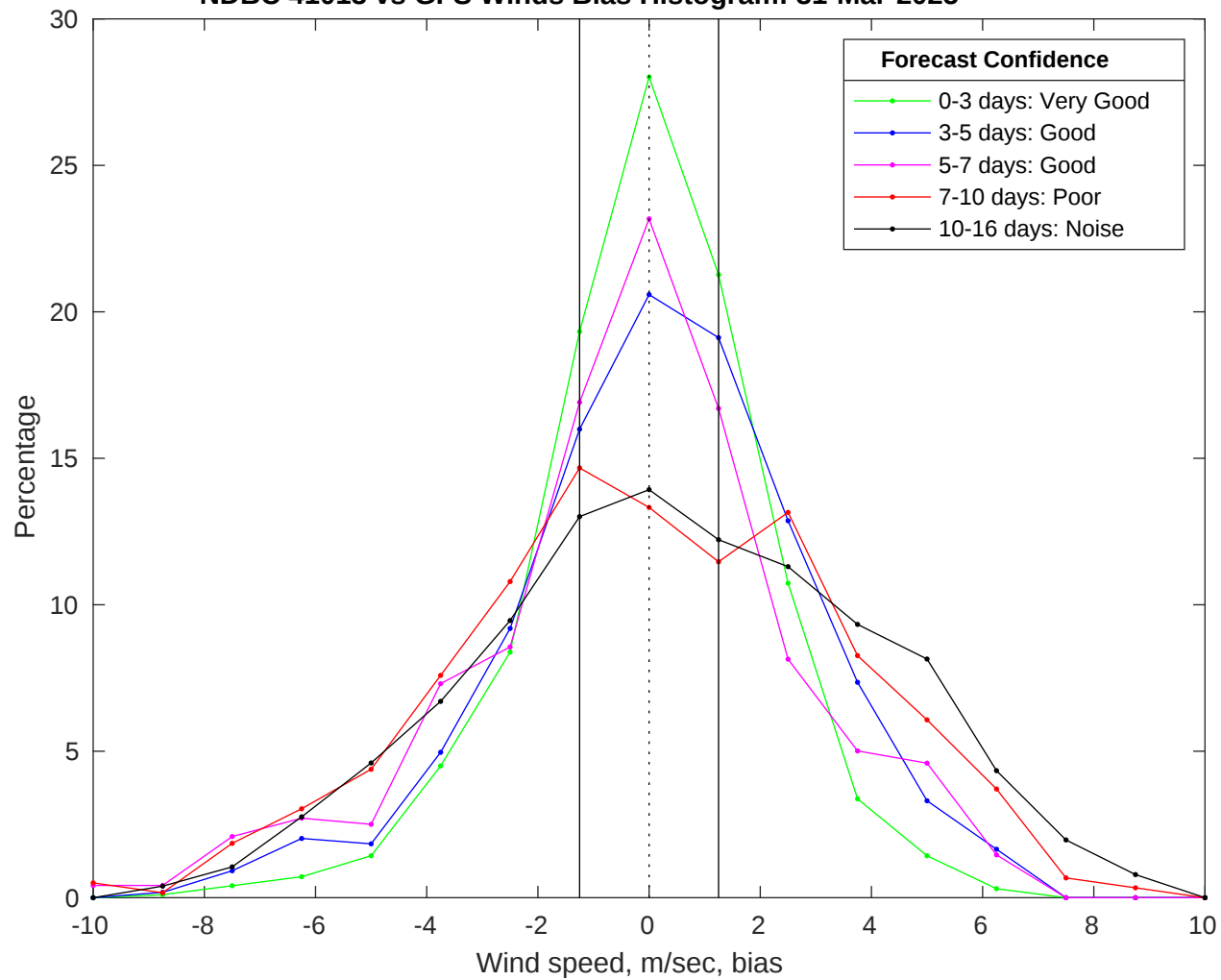
NDBC 41013 vs GFS Winds Bias Histogram: 31-Mar-2025
