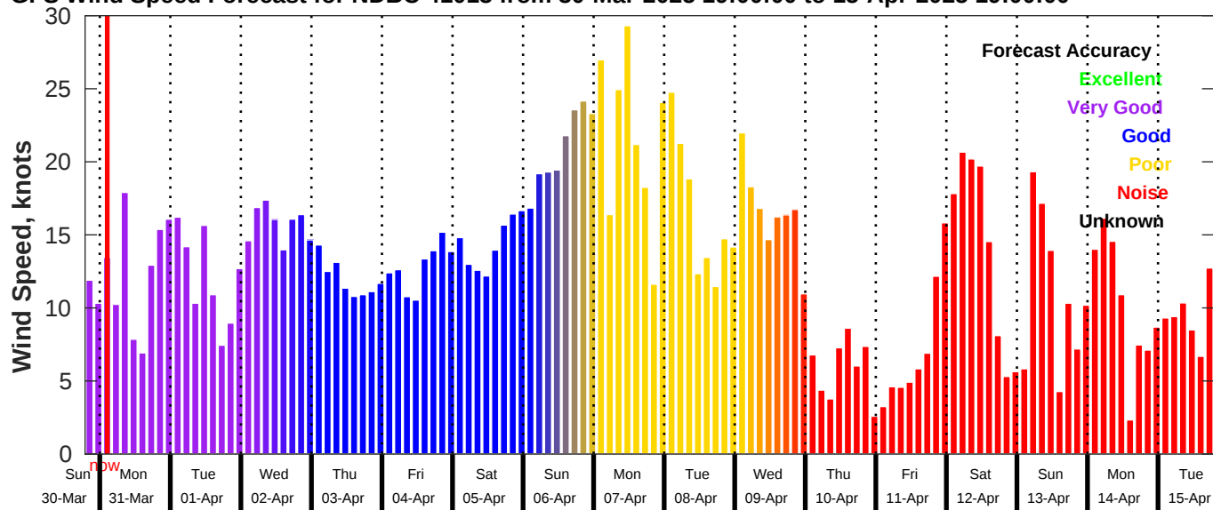
GFS Wind Speed Forecast for NDBC 41013 from 30-Mar-2025 19:00:00 to 15-Apr-2025 19:00:00
