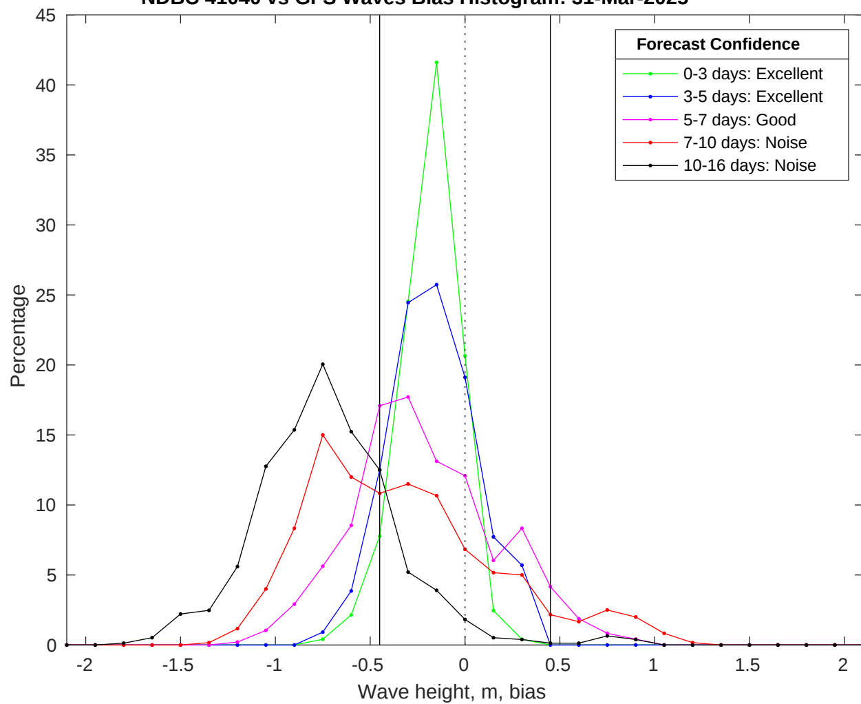
NDBC 41040 vs GFS Waves Bias Histogram: 31-Mar-2025
