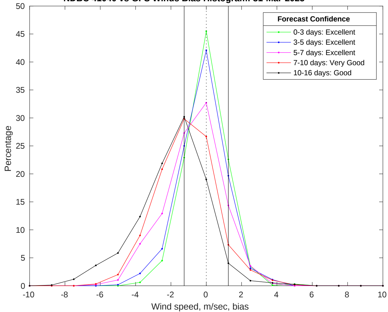
NDBC 41040 vs GFS Winds Bias Histogram: 31-Mar-2025
