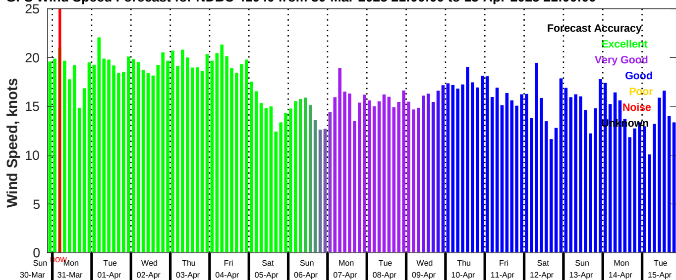
GFS Wind Speed Forecast for NDBC 41040 from 30-Mar-2025 21:00:00 to 15-Apr-2025 21:00:00
