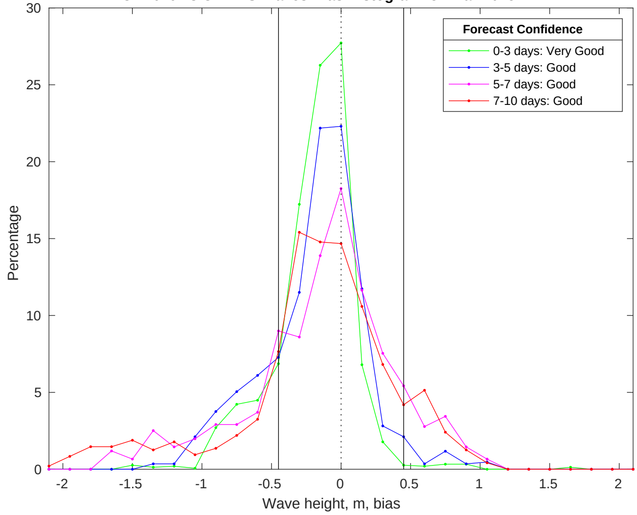
NDBC 42019 vs CMEMS Waves Bias Histogram: 31-Mar-2025
