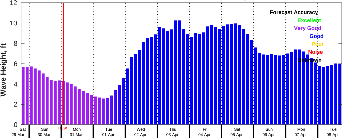
CMEMS Wave Forecast for NDBC 42019 from 29-Mar-2025 18:00:00 to 08-Apr-2025 18:00:00
