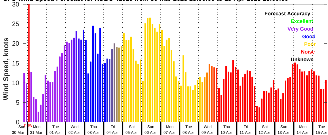
GFS Wind Speed Forecast for NDBC 42019 from 30-Mar-2025 18:00:00 to 15-Apr-2025 18:00:00
