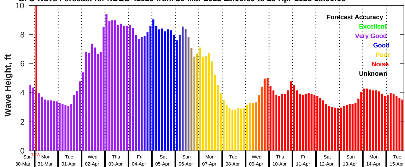
GFS Wave Forecast for NDBC 42020 from 30-Mar-2025 18:00:00 to 15-Apr-2025 18:00:00
