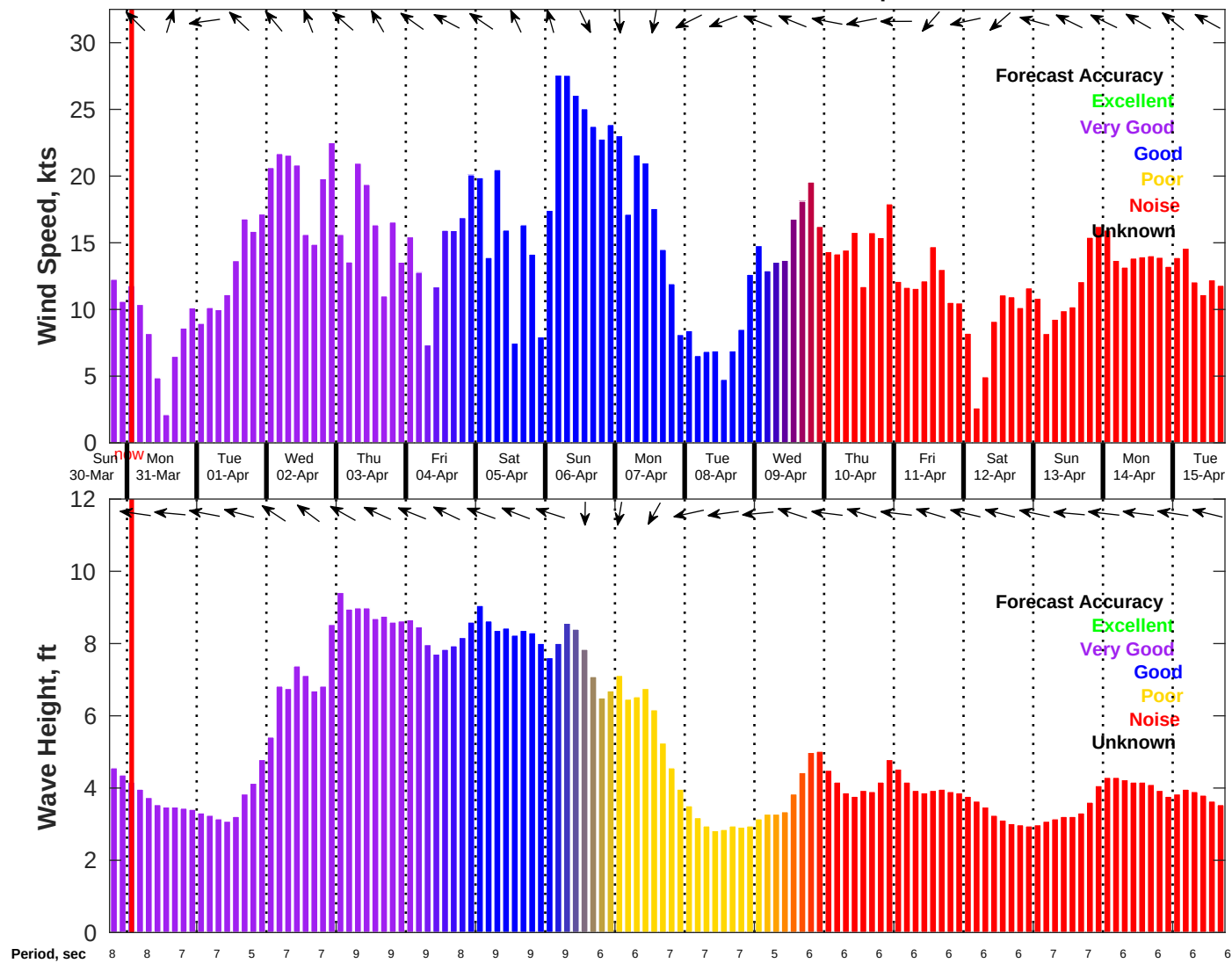
Wind & Wave Forecast for NDBC 42020 from 30-Mar-2025 18:00:00 to 15-Apr-2025 18:00:00
