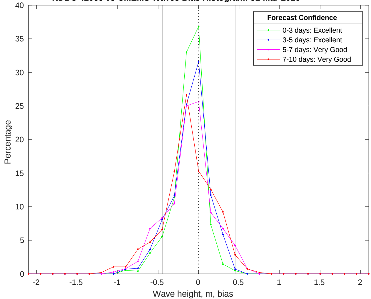
NDBC 42035 vs CMEMS Waves Bias Histogram: 31-Mar-2025
