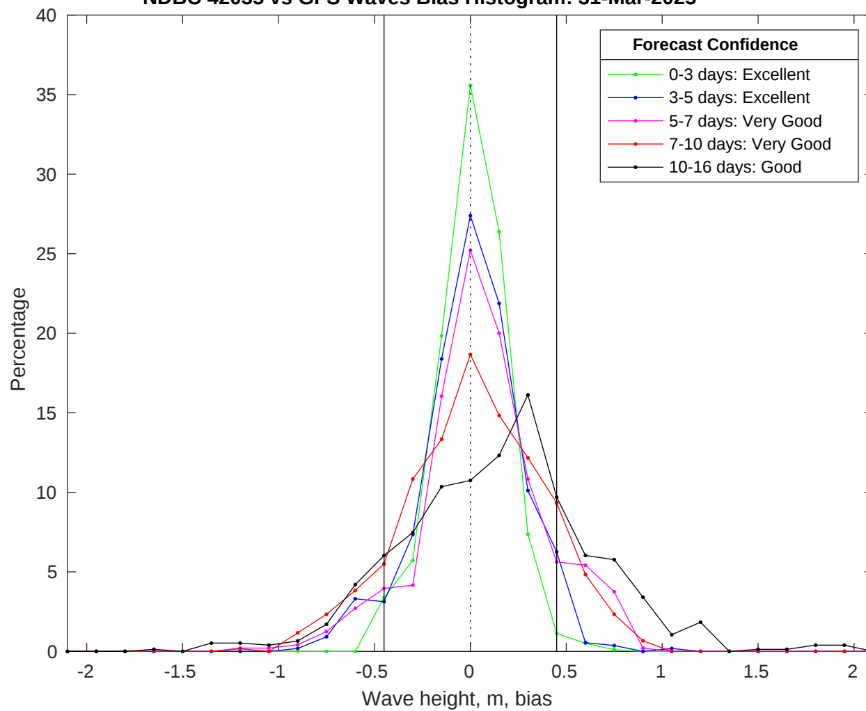
NDBC 42035 vs GFS Waves Bias Histogram: 31-Mar-2025
