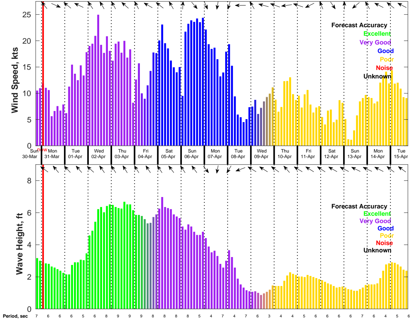
Wind & Wave Forecast for NDBC 42035 from 30-Mar-2025 18:00:00 to 15-Apr-2025 18:00:00
