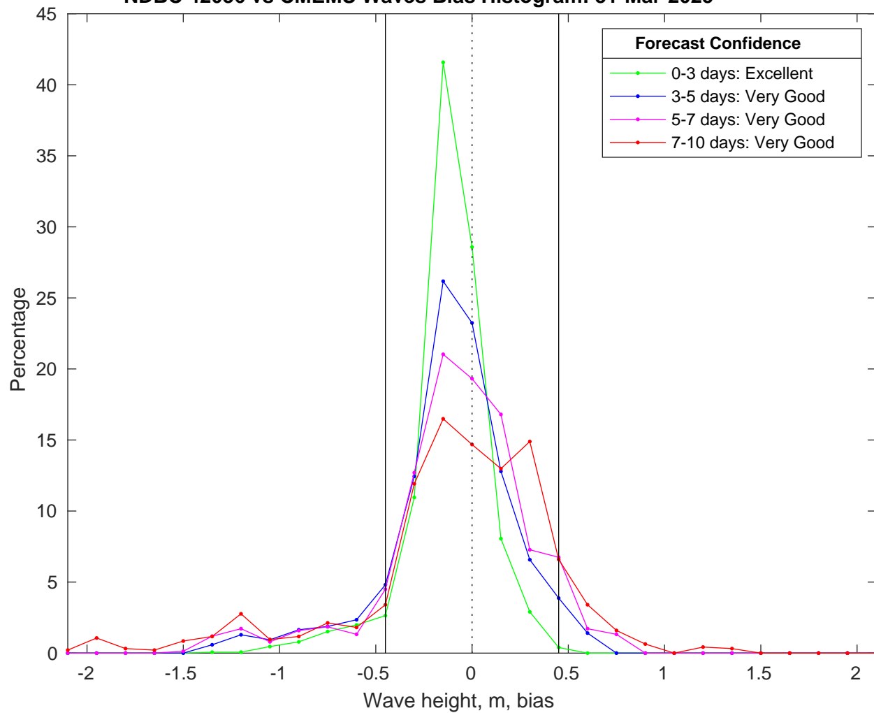
NDBC 42036 vs CMEMS Waves Bias Histogram: 31-Mar-2025
