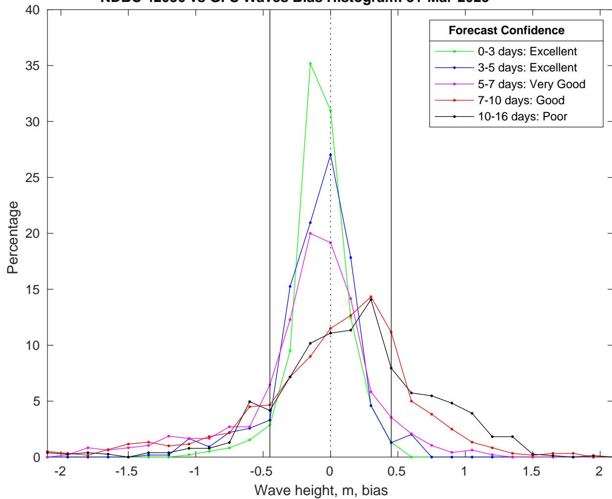
NDBC 42036 vs GFS Waves Bias Histogram: 31-Mar-2025
