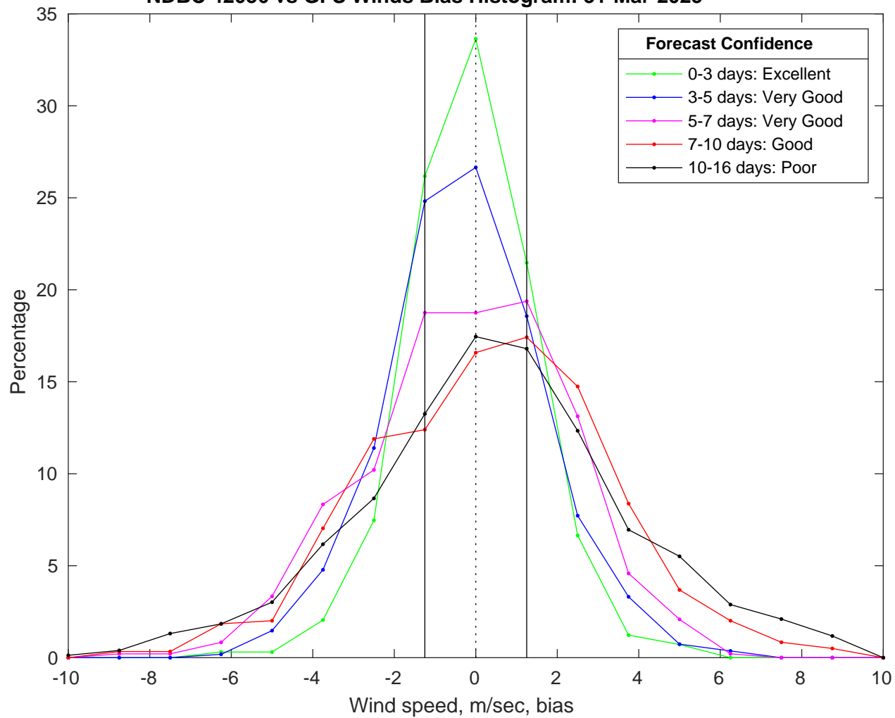
NDBC 42036 vs GFS Winds Bias Histogram: 31-Mar-2025
