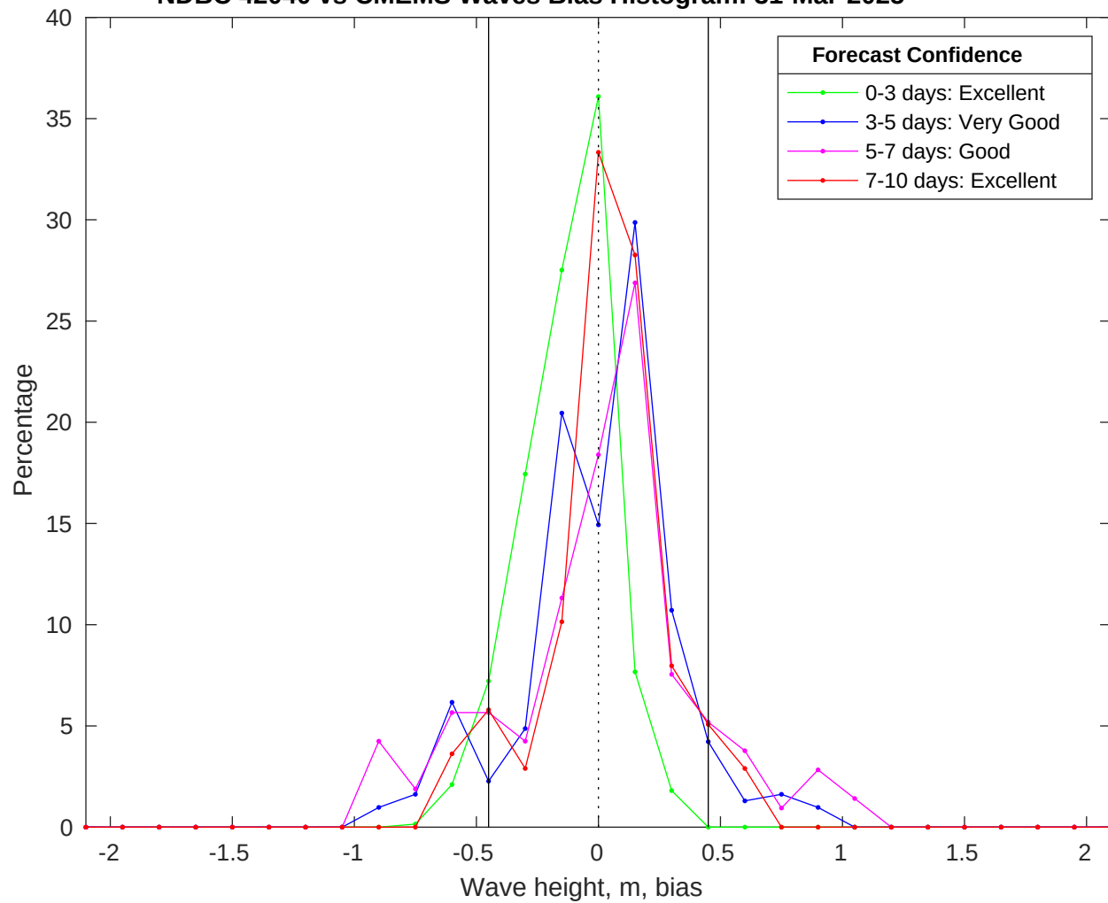
NDBC 42040 vs CMEMS Waves Bias Histogram: 31-Mar-2025
