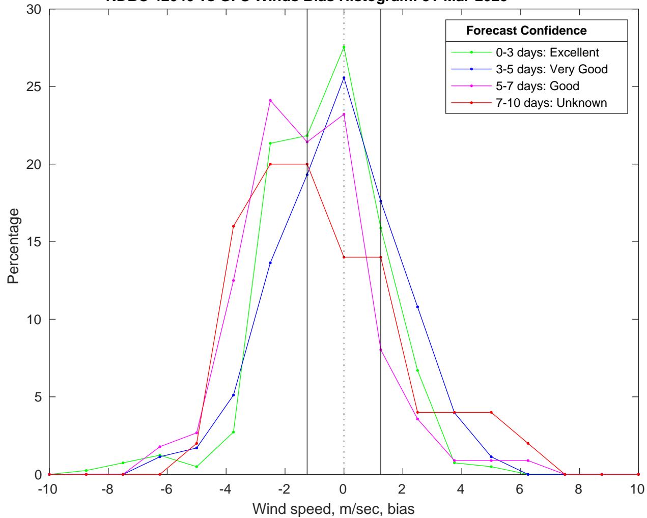
NDBC 42040 vs GFS Winds Bias Histogram: 31-Mar-2025
