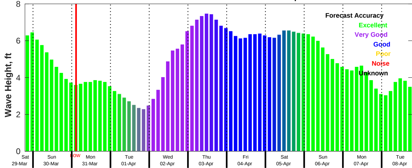
CMEMS Wave Forecast for NDBC 42040 from 29-Mar-2025 19:00:00 to 08-Apr-2025 19:00:00
