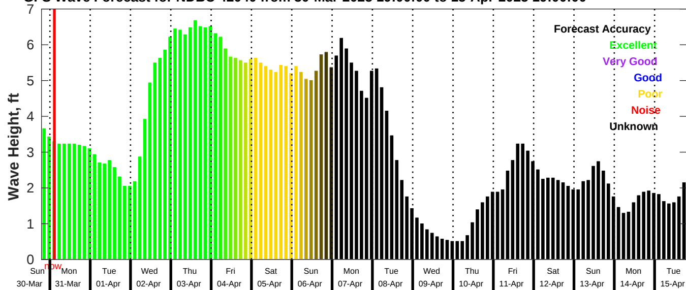
GFS Wave Forecast for NDBC 42040 from 30-Mar-2025 19:00:00 to 15-Apr-2025 19:00:00
