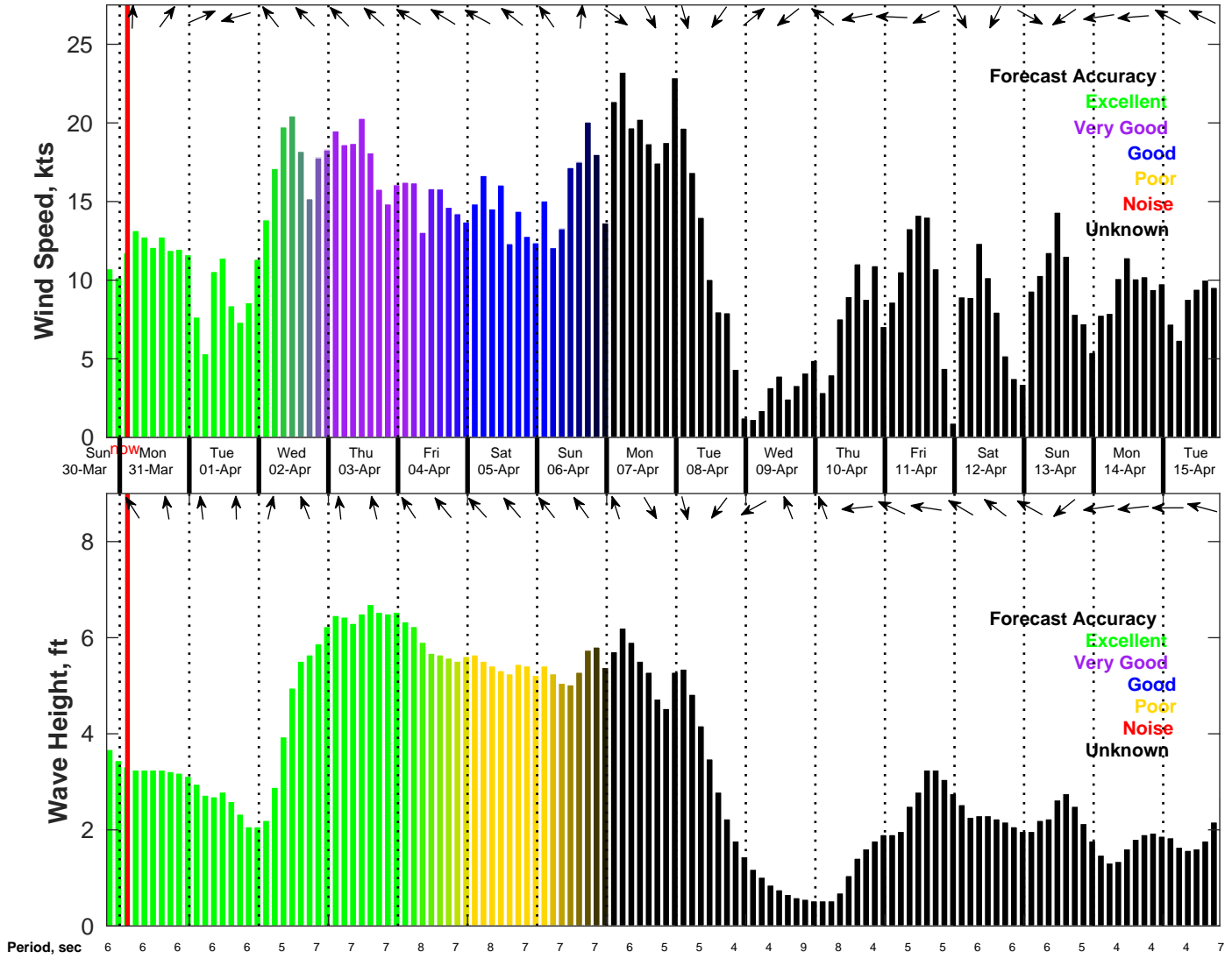
Wind & Wave Forecast for NDBC 42040 from 30-Mar-2025 19:00:00 to 15-Apr-2025 19:00:00
