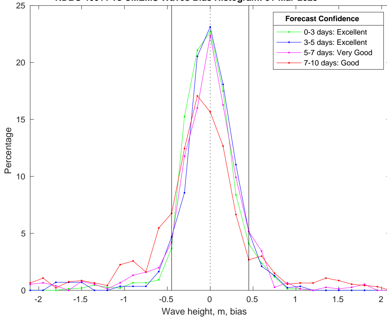
NDBC 46011 vs CMEMS Waves Bias Histogram: 31-Mar-2025
