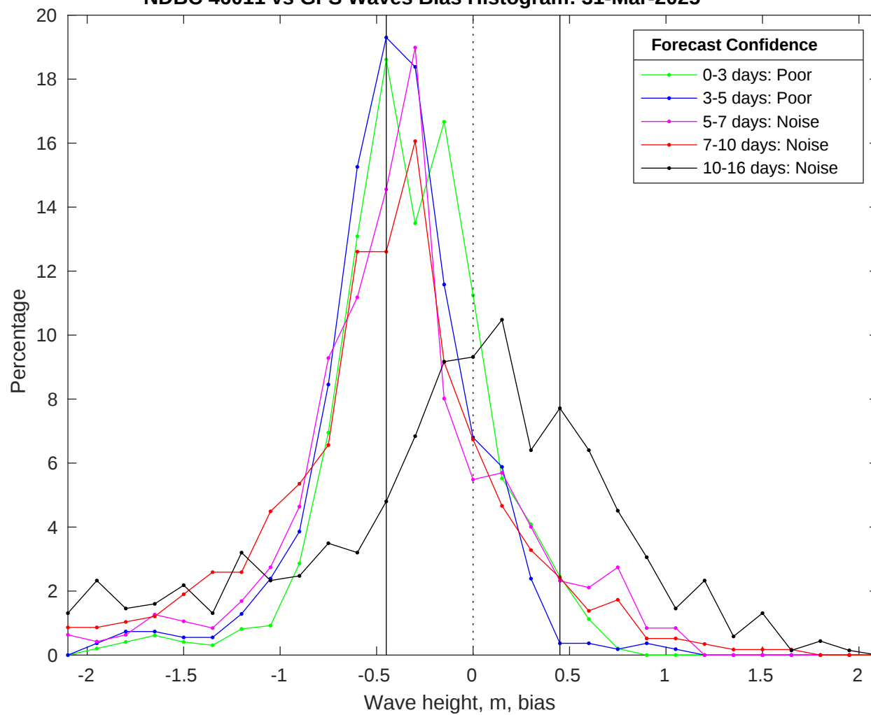
NDBC 46011 vs GFS Waves Bias Histogram: 31-Mar-2025
